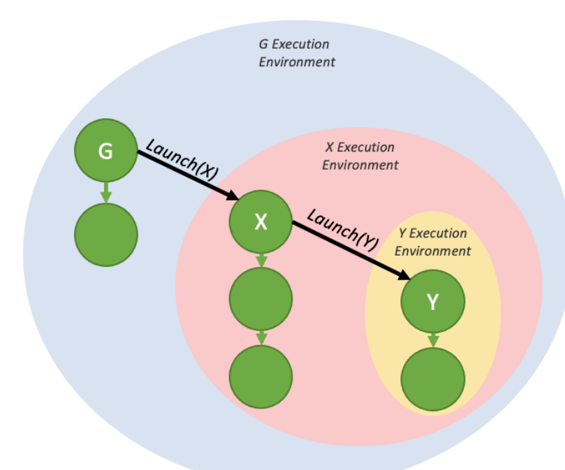
Figure 17: Nested fire and forget environments
