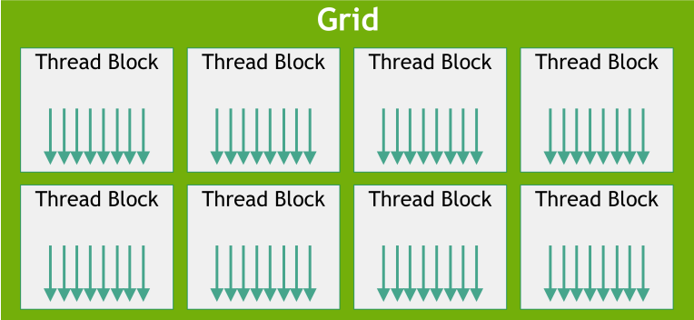
Figure 4: Grid of Thread Blocks
