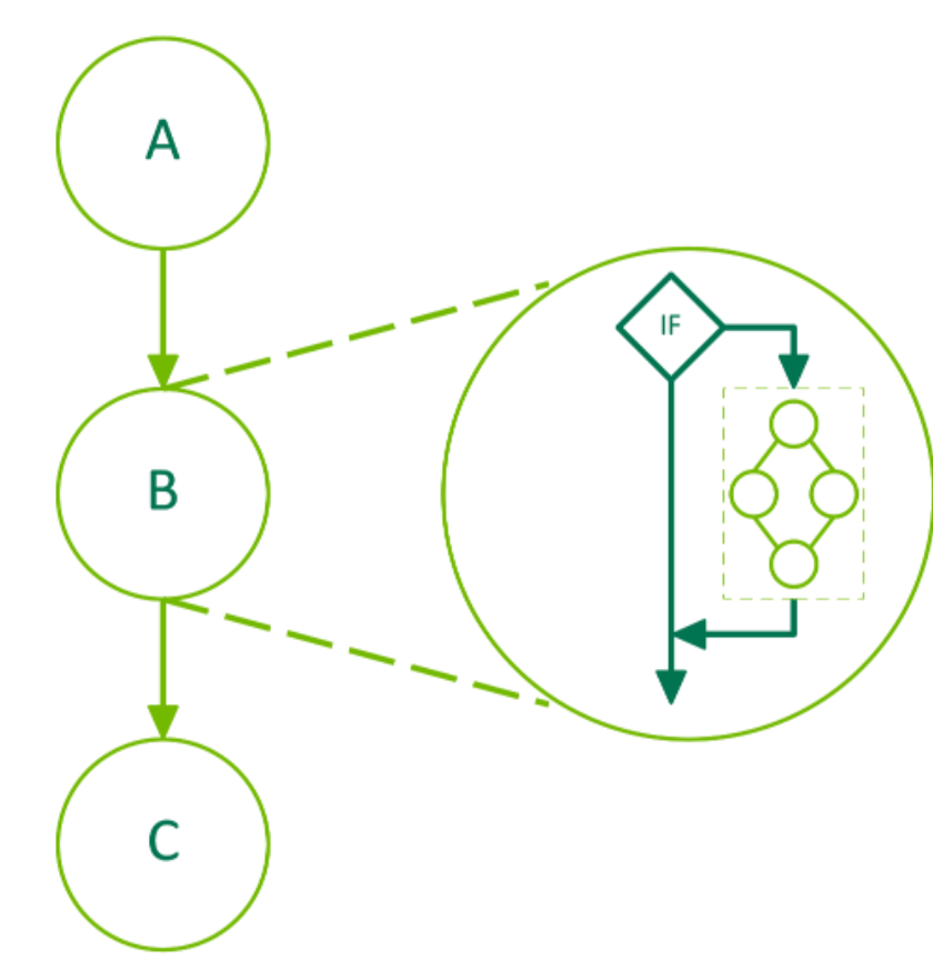
Figure 23: Conditional IF Node
