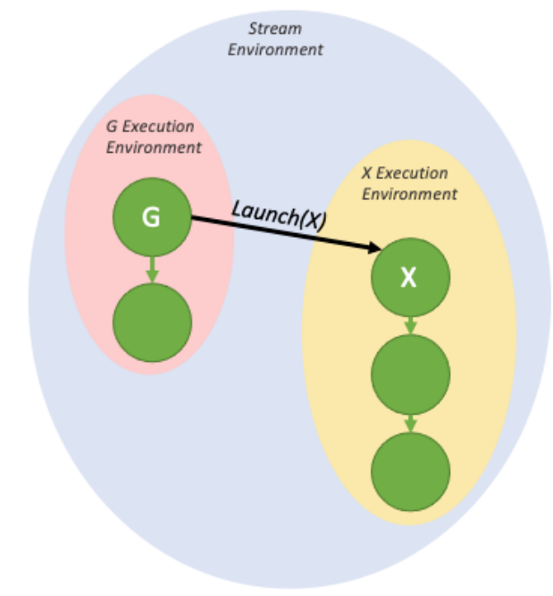
Figure 22: A simple sibling launch
