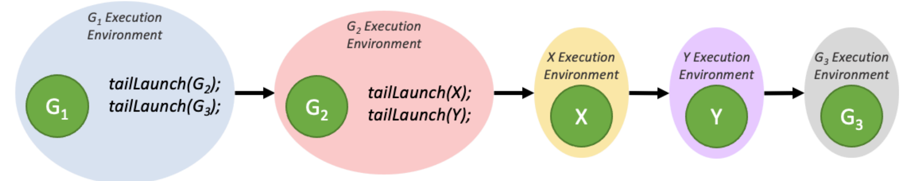
Figure 21: Tail launch ordering when enqueued from multiple graphs
