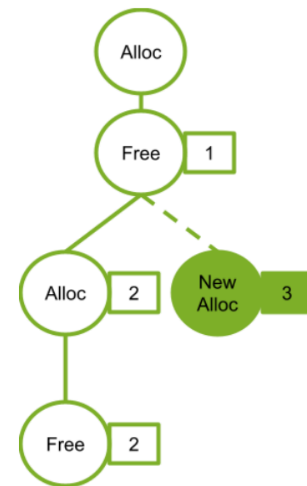
Figure 30: Adding New Alloc Node 3
