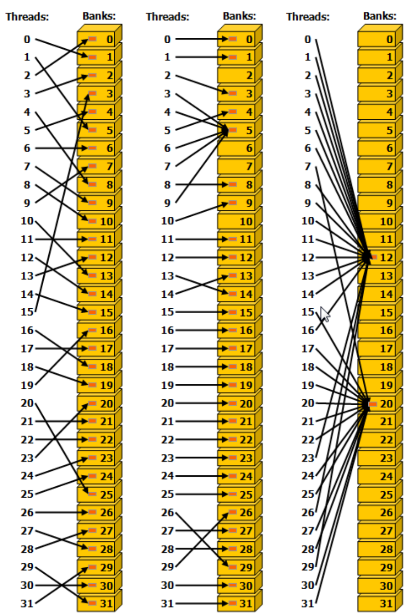
Figure 36: Irregular Shared Memory Accesses.
