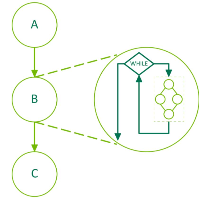
Figure 24: Conditional WHILE Node
