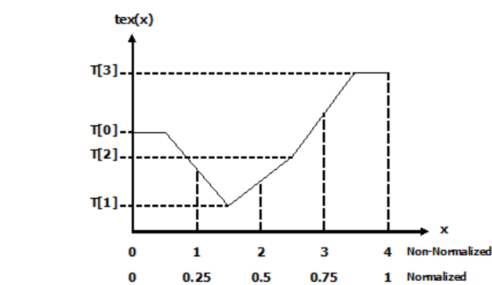
Figure 33: Linear Filtering Mode
