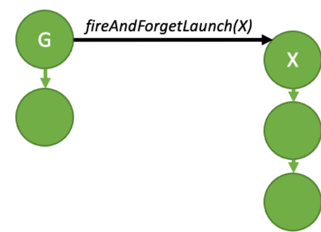
Figure 15: Fire and forget launch
