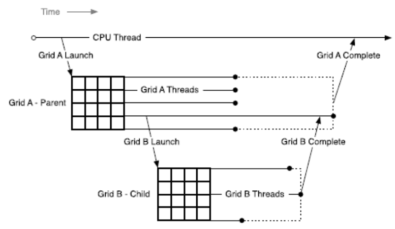
Figure 26: Parent-Child Launch Nesting
