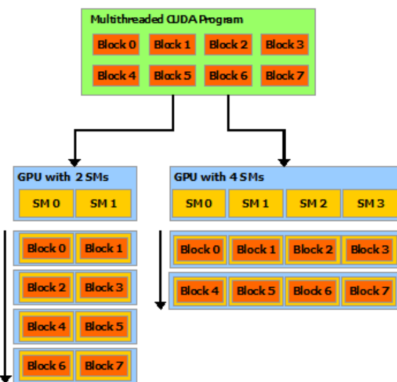
Figure 3: Automatic Scalability
