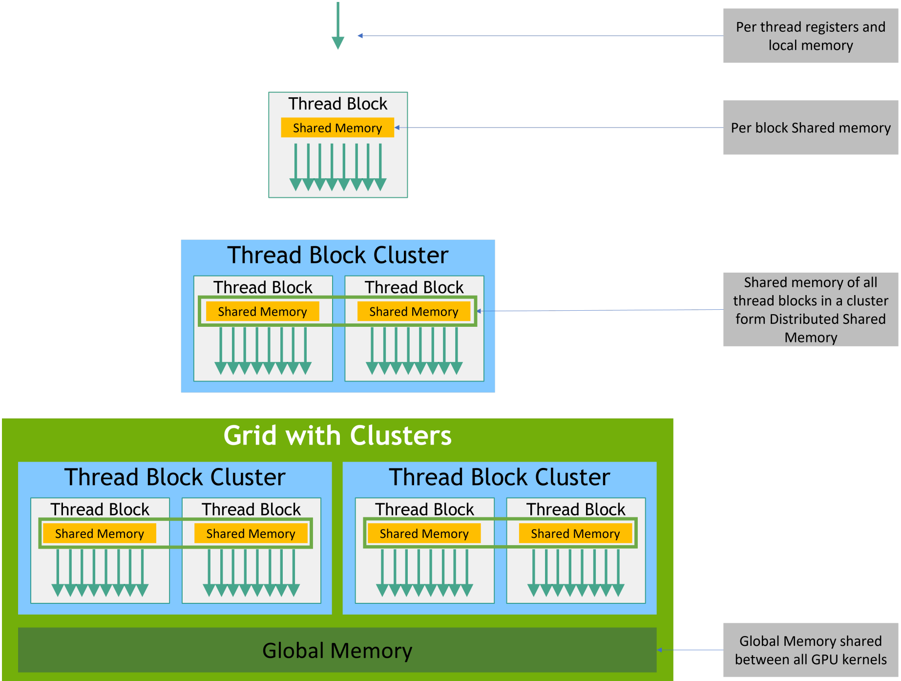
Figure 6: Memory Hierarchy
