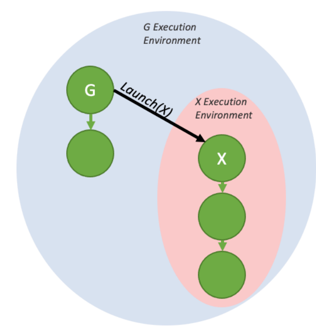
Figure 16: Fire and forget launch, with execution environments
