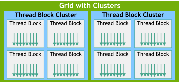
Figure 5: Grid of Thread Block Clusters
