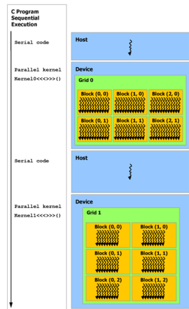
Figure 7: Heterogeneous Programming
