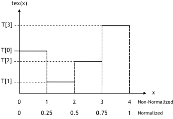
Figure 32: Nearest-Point Sampling Filtering Mode
