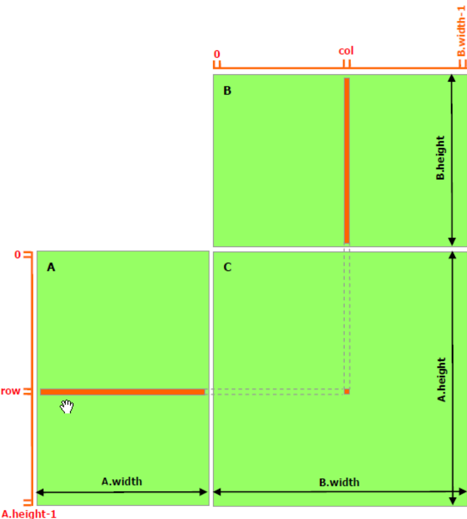
Figure 8: Matrix Multiplication without Shared Memory
