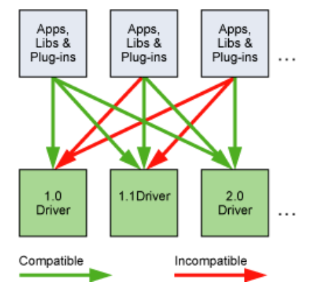
Figure 25: The Driver API is Backward but Not Forward Compatible
