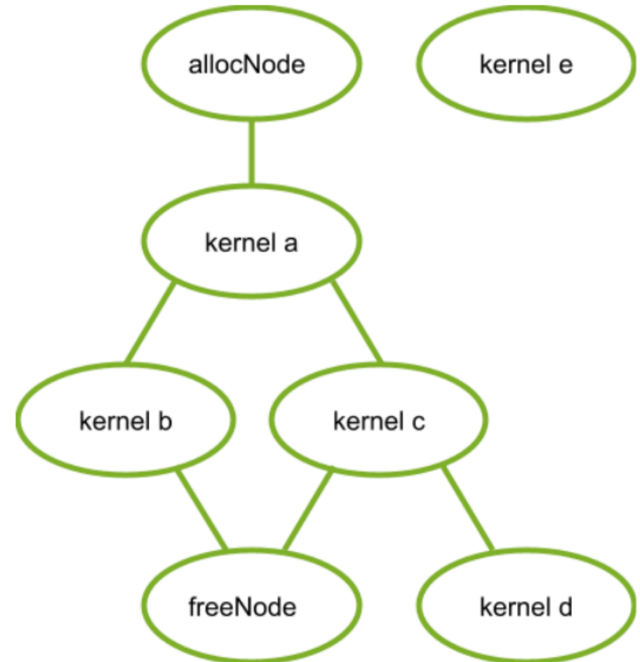
Figure 28: Kernel Nodes
