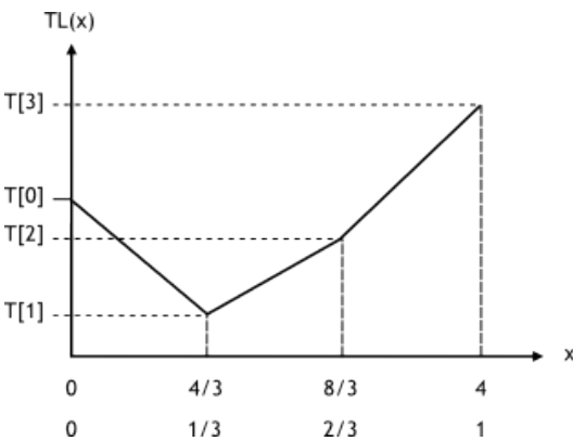
Figure 34: One-Dimensional Table Lookup Using Linear Filtering
