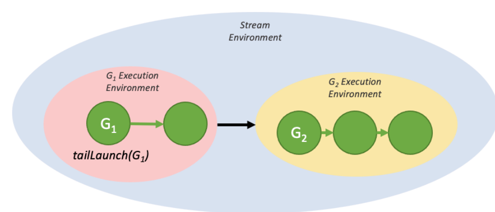
Figure 19: A simple tail launch
