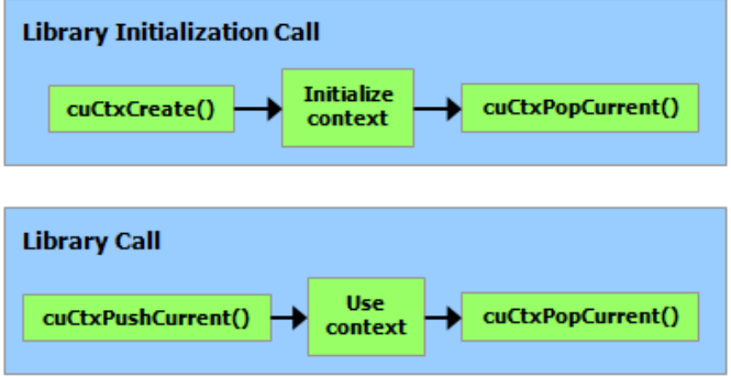
Figure 37: Library Context Management
