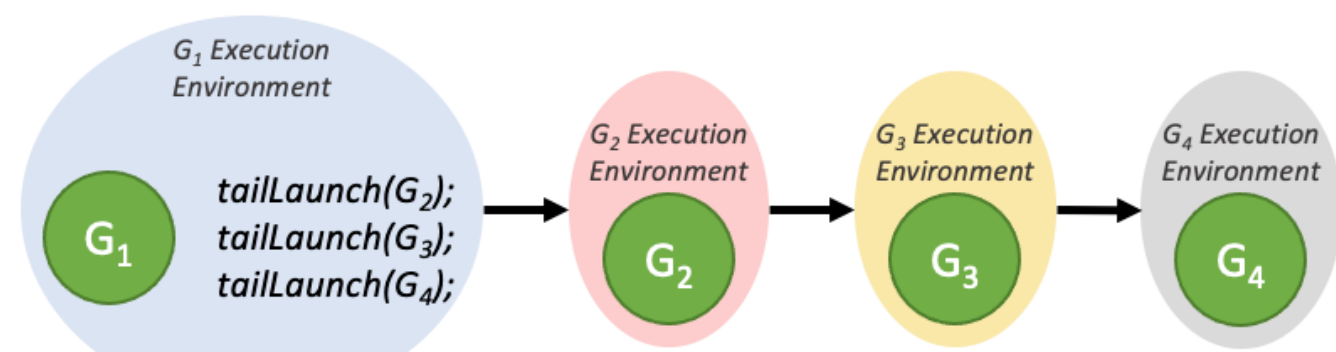
Figure 20: Tail launch ordering
